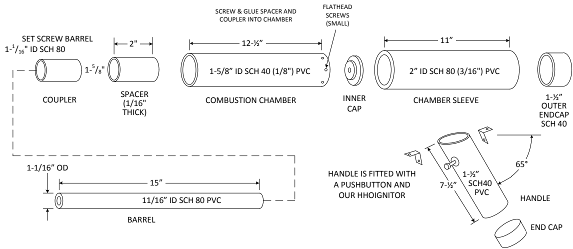
Figure 18-10: Overall Assembly
