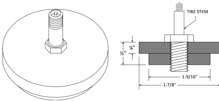
Figure 18-4: Tire Stem in Inner Cap
