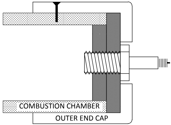
Figure 18-8: Hole Through End Cap Sides
