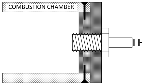
Figure 18-7: Holes Through Sides
