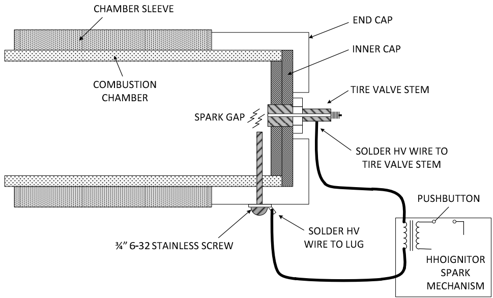
Figure 18-12: Wiring
