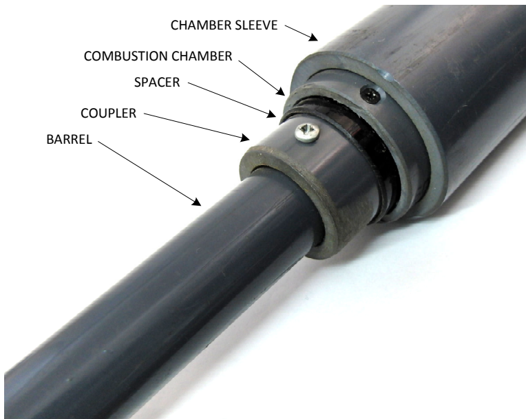
Figure 18-11: Detail of Chamber Stepping Down to Barrel
