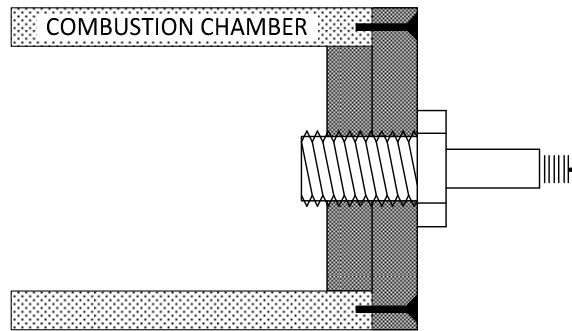
Figure 18-6: Holes Through Bottom
