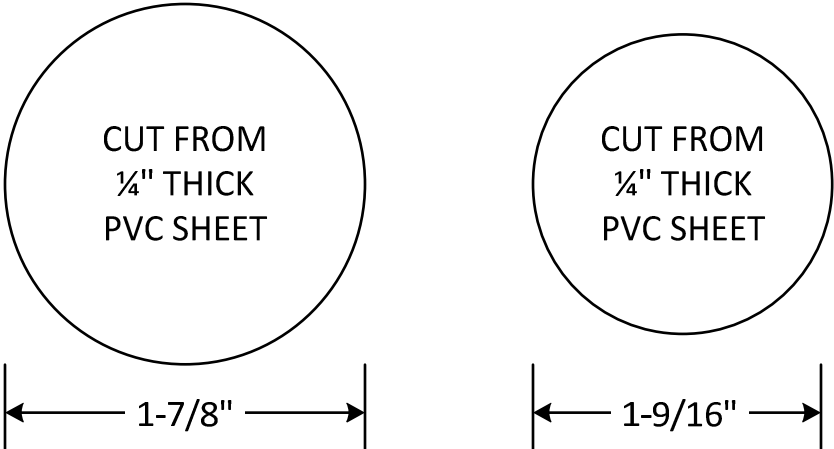
Figure 18-2: Inner Cap Pieces
