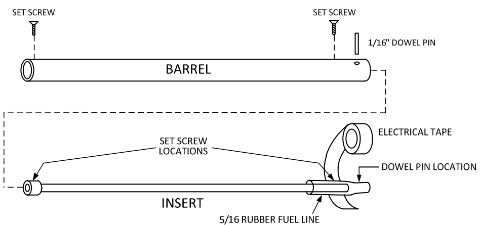
Figure 18-9: Barrel Assembly
