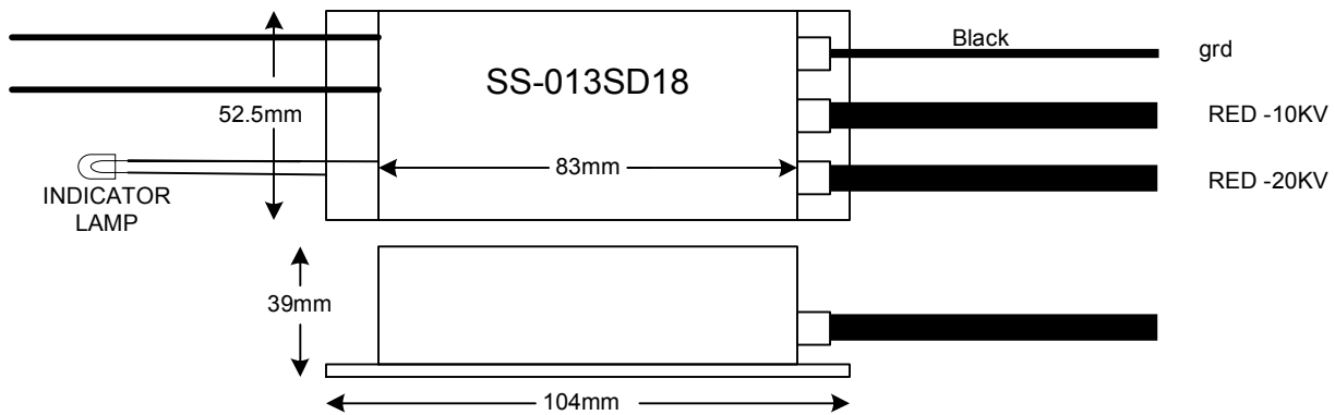
Schematic
