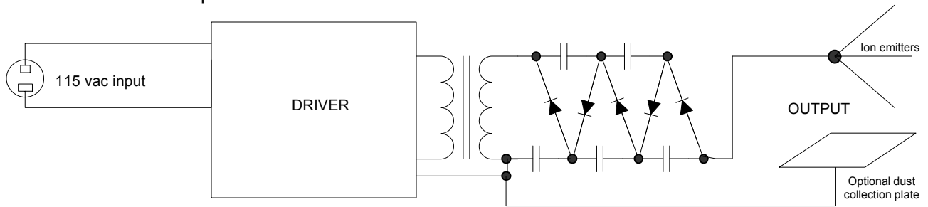
Schematic
